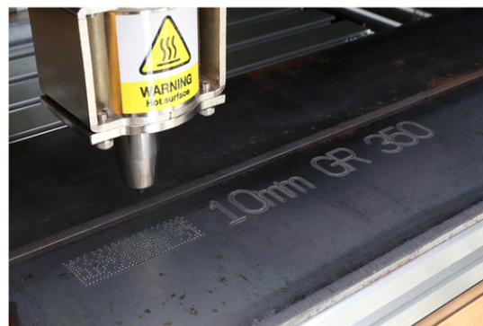
Big Solenoid (BSD) for deeper marking is attachable.
